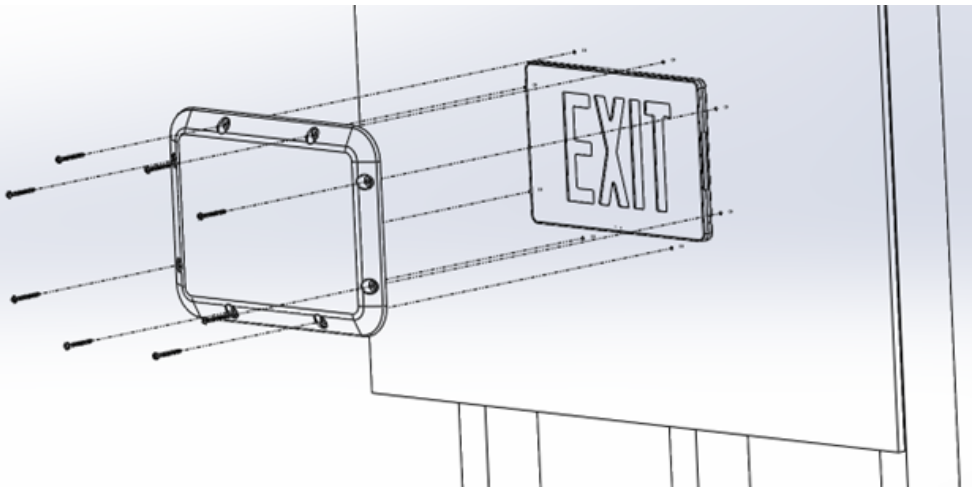
FIGURE 3: BACK MOUNT WITH FRAMED SUPPORT
