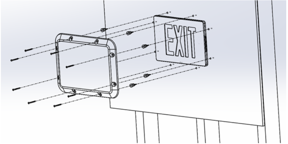
FIGURE 1: BACK MOUNT WITH ANCHORS
