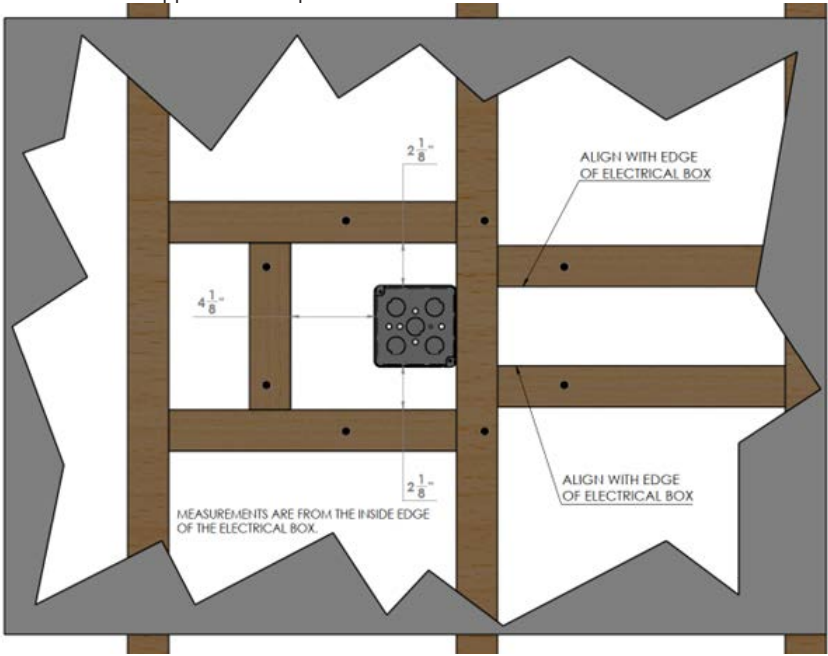
FIGURE 2: FRAMED SUPPORT
