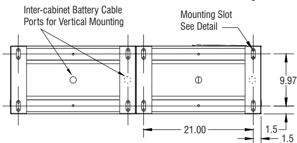
Floor Mounting Bolt Pattern
