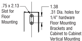
Mounting Slot Detail
