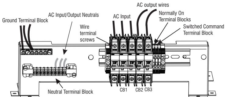
Optional Output Circuit Breaker Illustration
