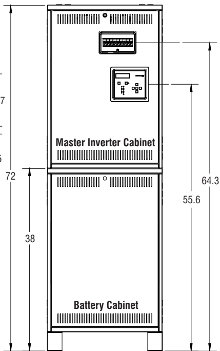
Vertical Mounting
